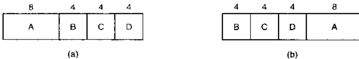
Figure 2-39. An example of shortest job first scheduling. (a) Running four jobs in the original order. (b) Running them in shortest job first order.
